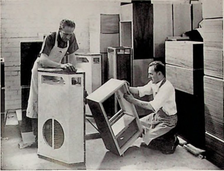
FIG. 7/2. Staining and filling cabinet surfaces in one operation.
