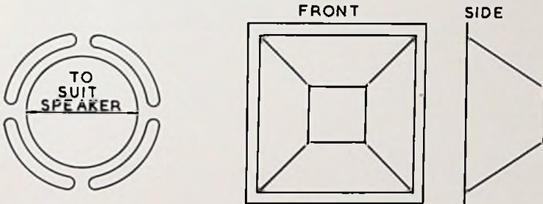
FIG. 13/4. Tweeter box with sloping sides to reflect sound through openings 1/2" wide, placed around the speaker. Line with thin layer of absorbent material.
