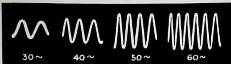
FIG. 12/2. Wave form with 8" RS unit in 1 cu.ft. enclosure with slotted back, placed 1" away from wall. Input 1 watt.
