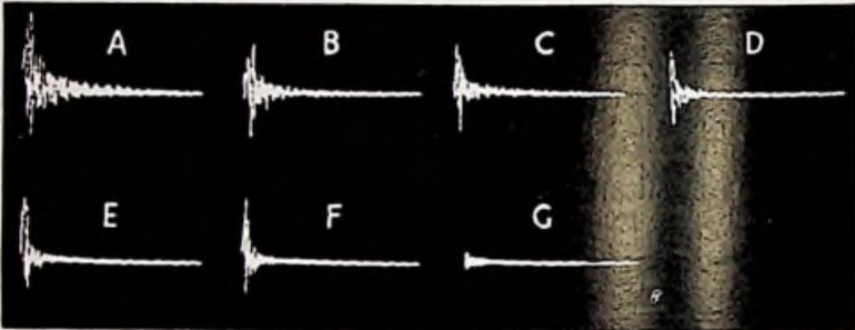
FIG. 9/1. Oscillograms showing vibration produced in 2' \times 2' panels by shock test. Time base 150 milliseconds.
