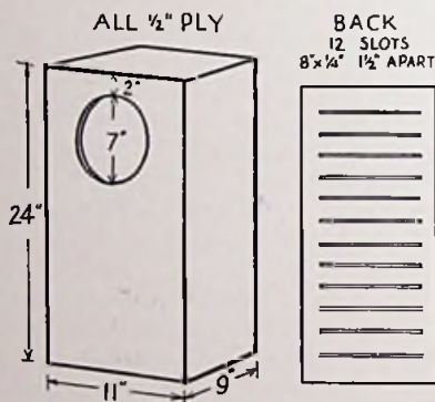
Fig. 12/3. DP Cabinet suitable for all types of 8" unit. Materials: \frac{1}{2} " plywood lined on all four sides with 1" absorbent. Back lined with soft woollen cloth. Weight: 14 lb. approx.
