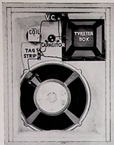
FIG. 13/5. Cabinet fitted with 12" and 3" units, reflecting box, volume control, 2.4 mH coil and 12 Mfd capacitor.
